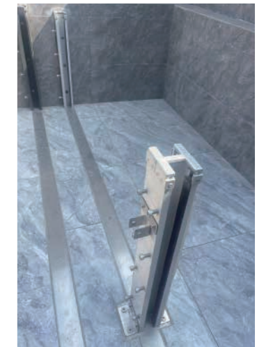
304 stainless steel base plate under aluminum flood barrier.
