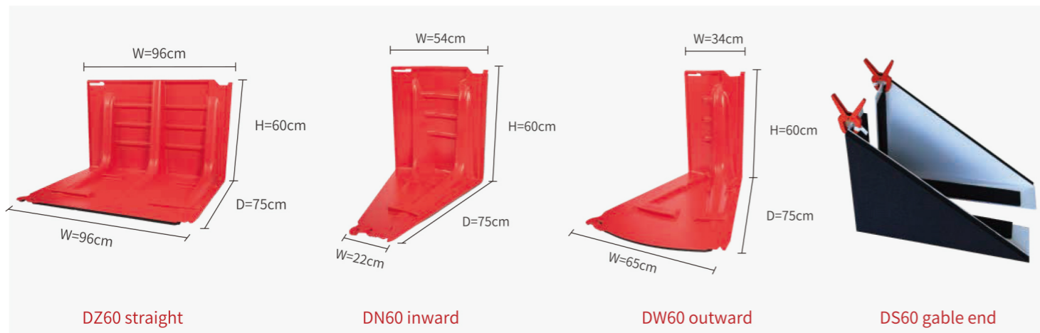
DZ50 straight DN50 inward DW50 outward DS50 gable end
